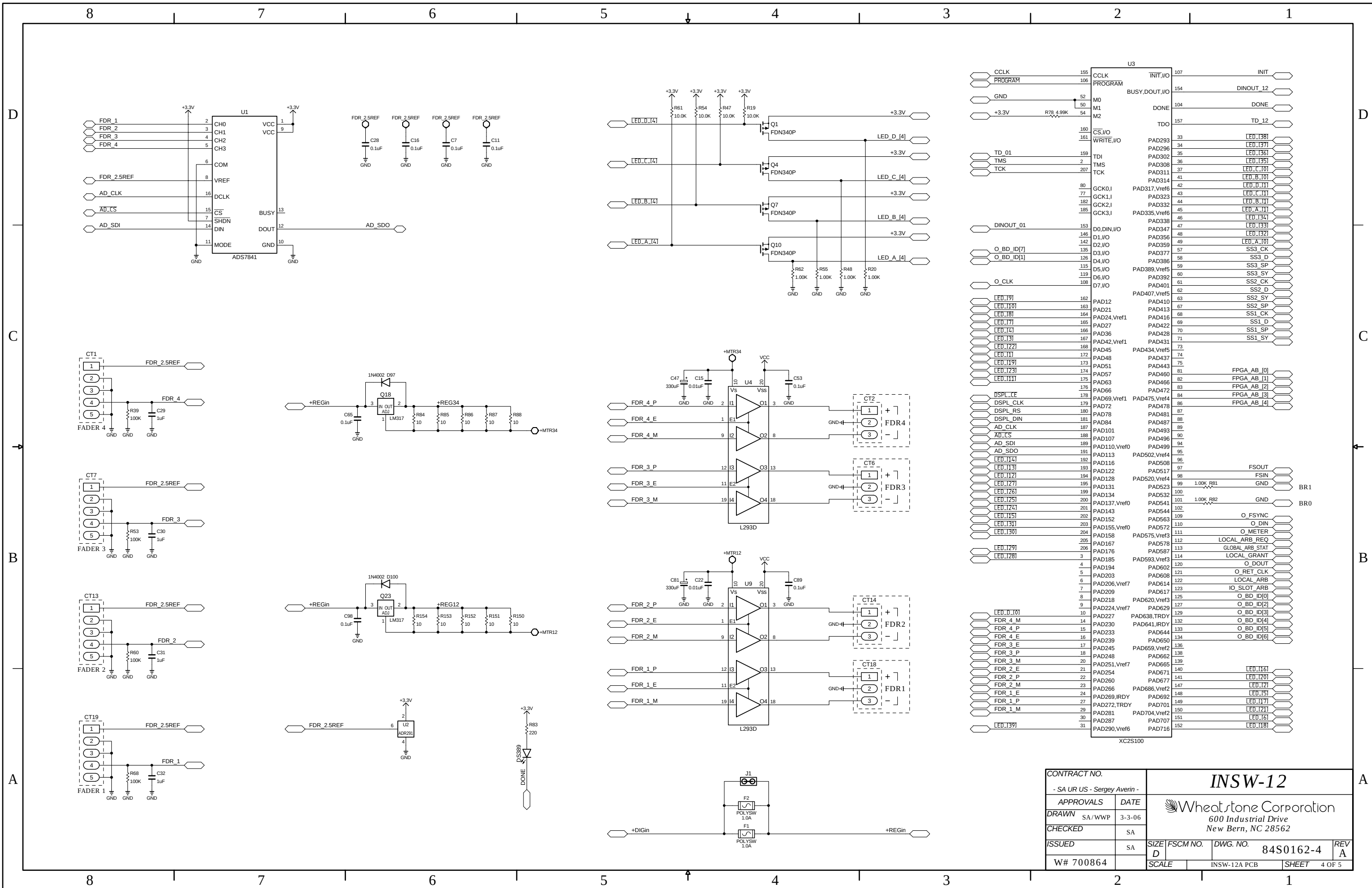
INSW-12 4 Inputs Panel Switch Card Schematic - Sheet 4 of 5
