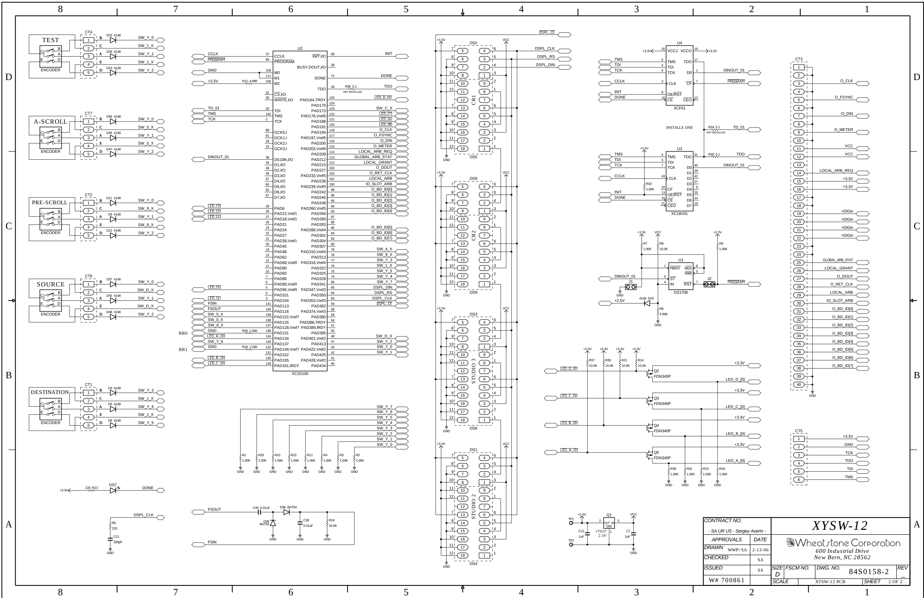
XYSW-12 Events Panel Switch Card Schematic - Sheet 2 of 2
