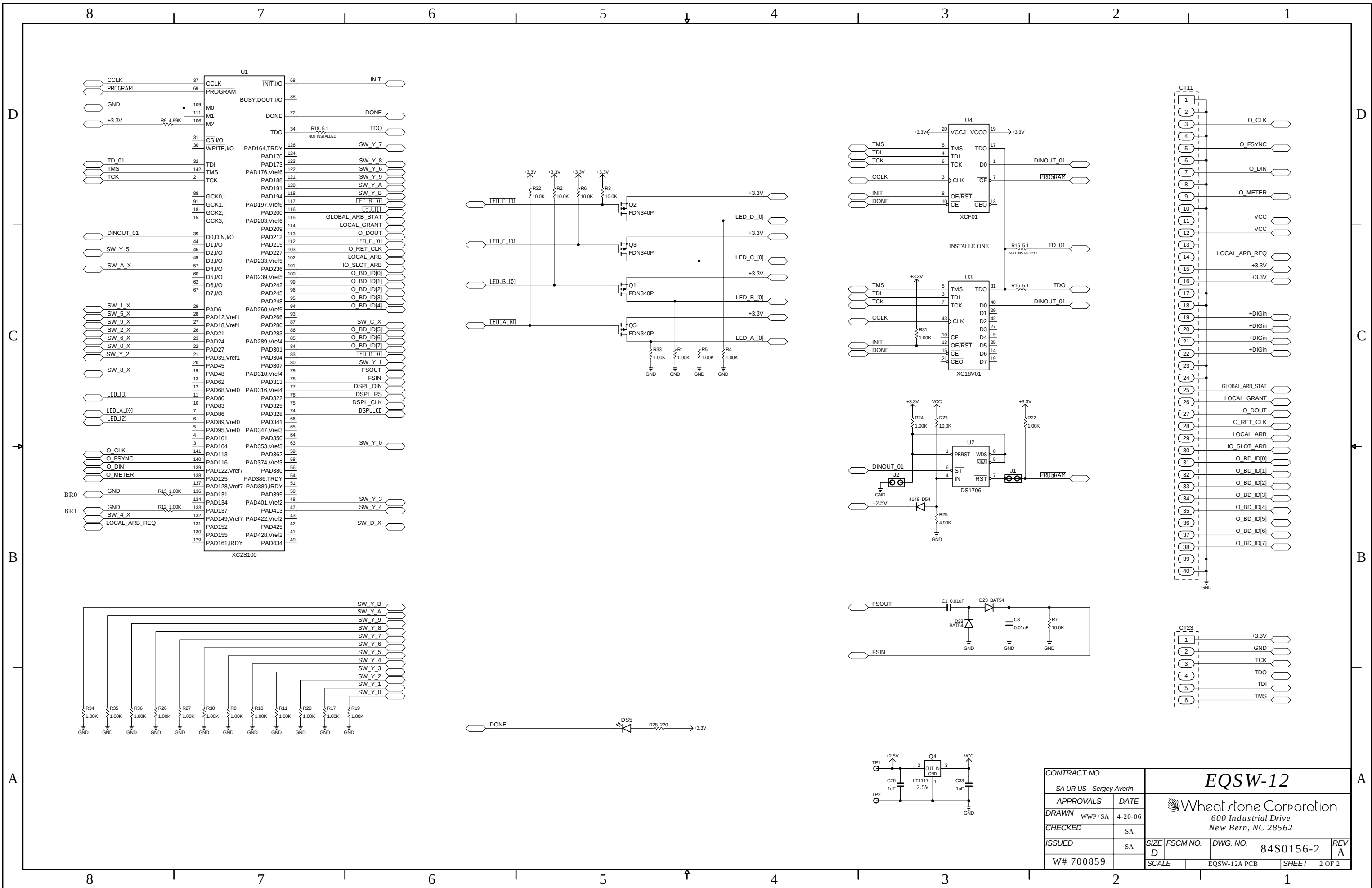
EQSW-12 EQ/Dynamics Panel Switch Card Schematic - Sheet 2 of 2
