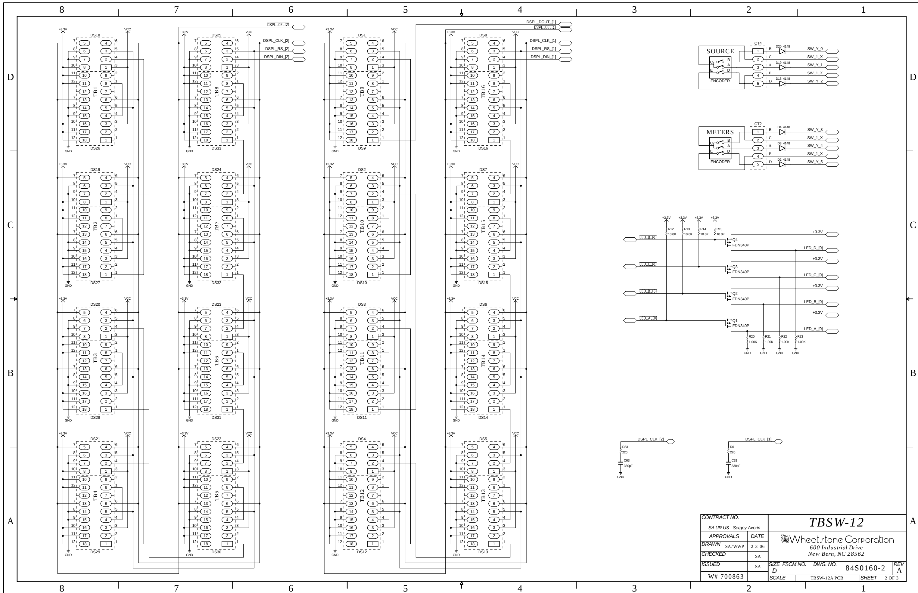
TBSW-12 Talkback Panel Switch Card Schematic - Sheet 2 of 3
